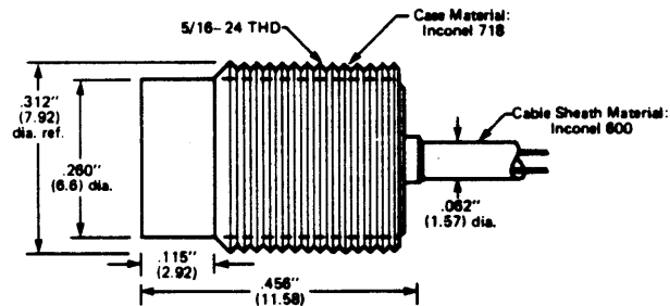
5/16-24 thread mount
