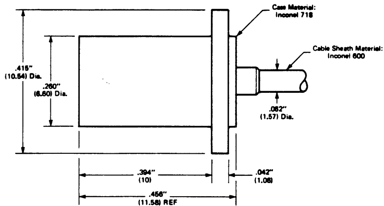
Flange mount, smooth body
