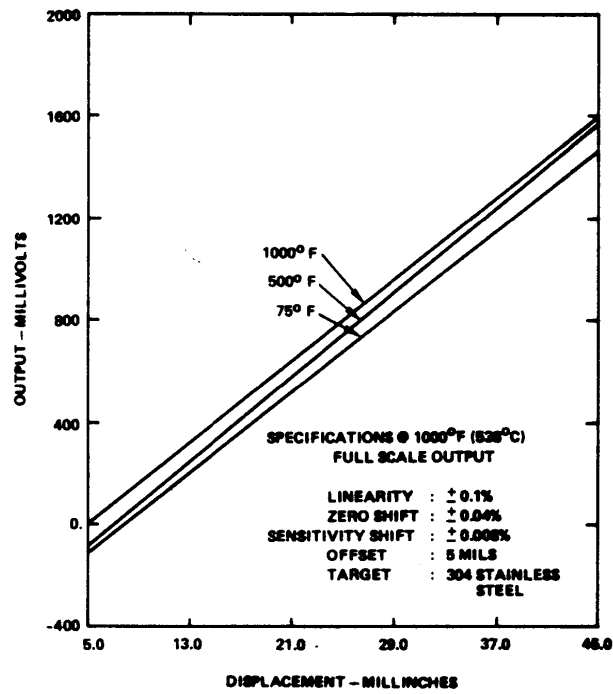
fig. 4 -- KD-1925 Performance
