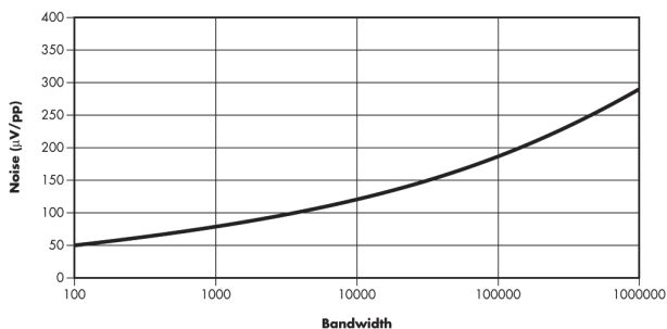
Typical Noise Performance: SMT9700 15N 100 Hz – 1 MHz
