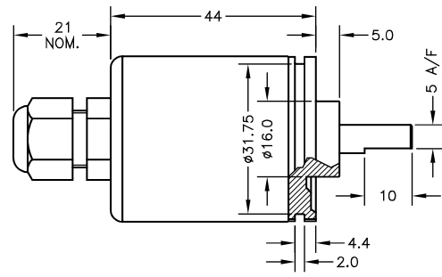
IP67 CABLE GLAND (CODE 'Lxx'/'LQxx')
