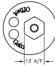
GAIN AND OFFSET ADJUSTMENTS SEALED (CODE 'Y')
