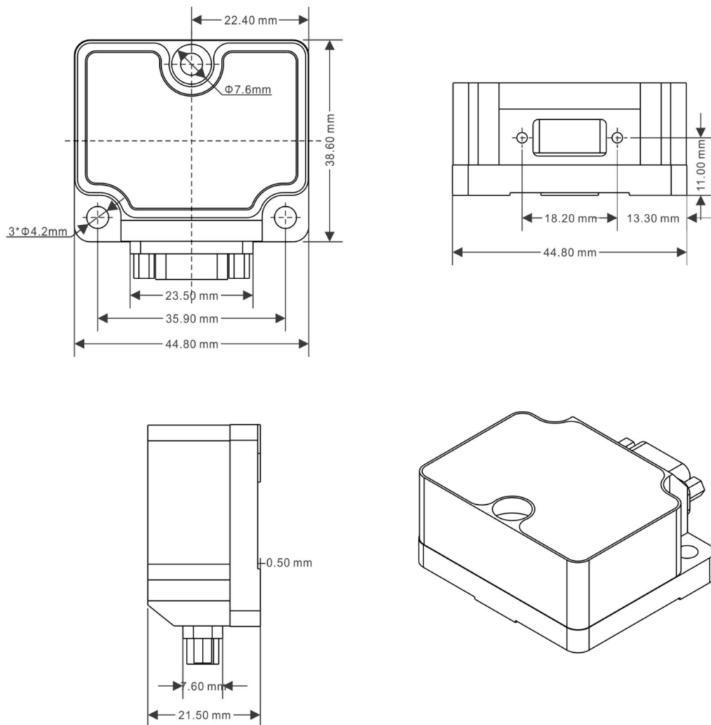
Fig. 4-1 Plug-in Node Configuration Diagram (Outside the Product)
