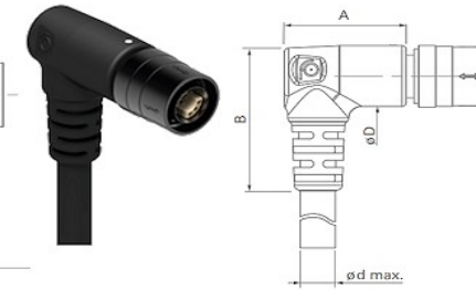
RIGHT-ANGLE OVERMOLDING
