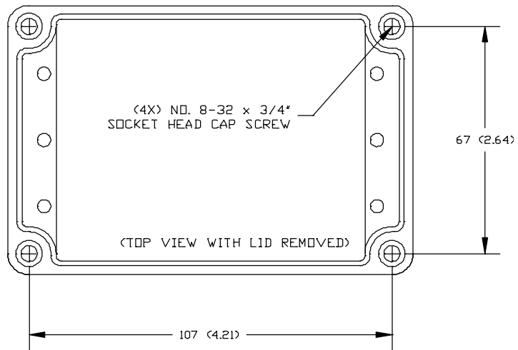
INSTRUMENT MOUNTING HOLE LOCATIONS DIMENSIONS: mm (in) Figure 5. Mounting Hole Pattern
