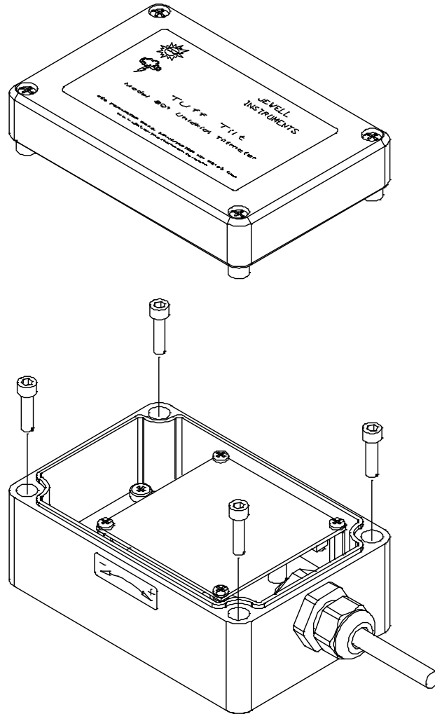
Figure 4. Mounting Screw Insertion
