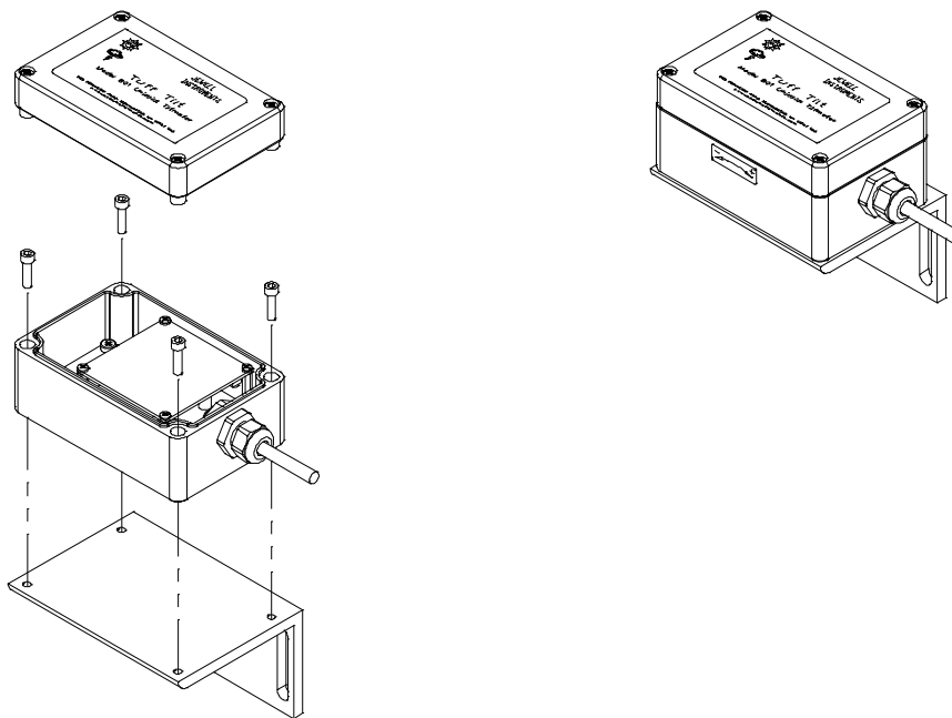
Figure 6. Using P/N 81439 Mounting Bracket
