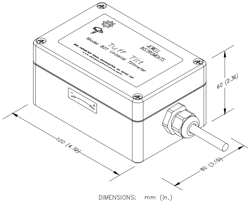
Figure 1. Model 801 Tiltmeter - Longitudinal Tilt Style
