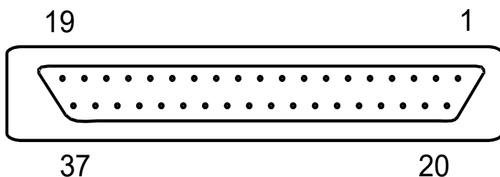
Terminal assignment 37 pin Sub D, female
