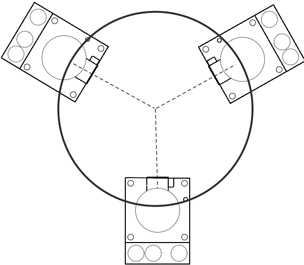
Circular system with three supporting points
