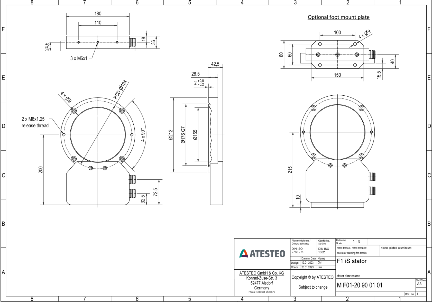
F1iS - Stator - no speed
