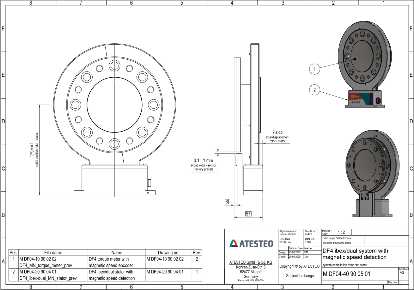
DF4 ibex - System - speed sensor
