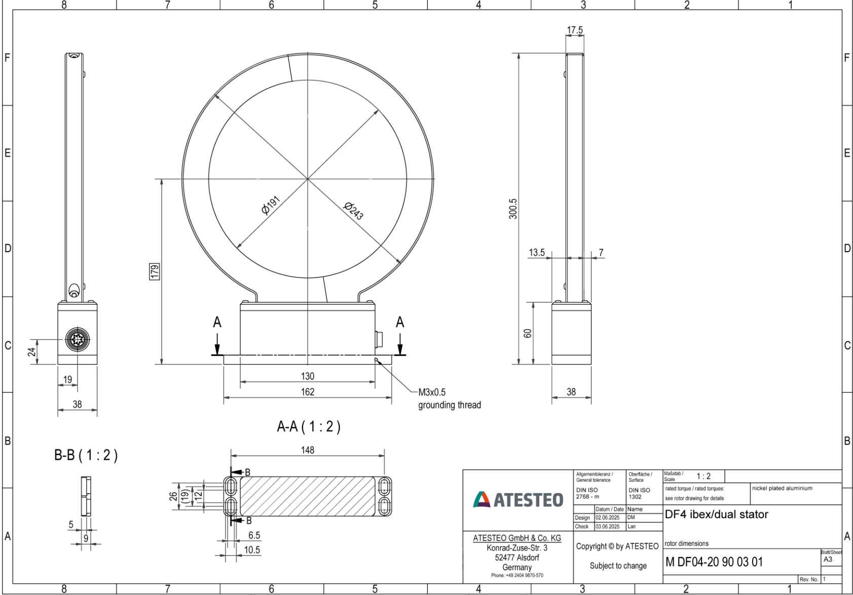
DF4 ibex - Stator - no speed sensor
