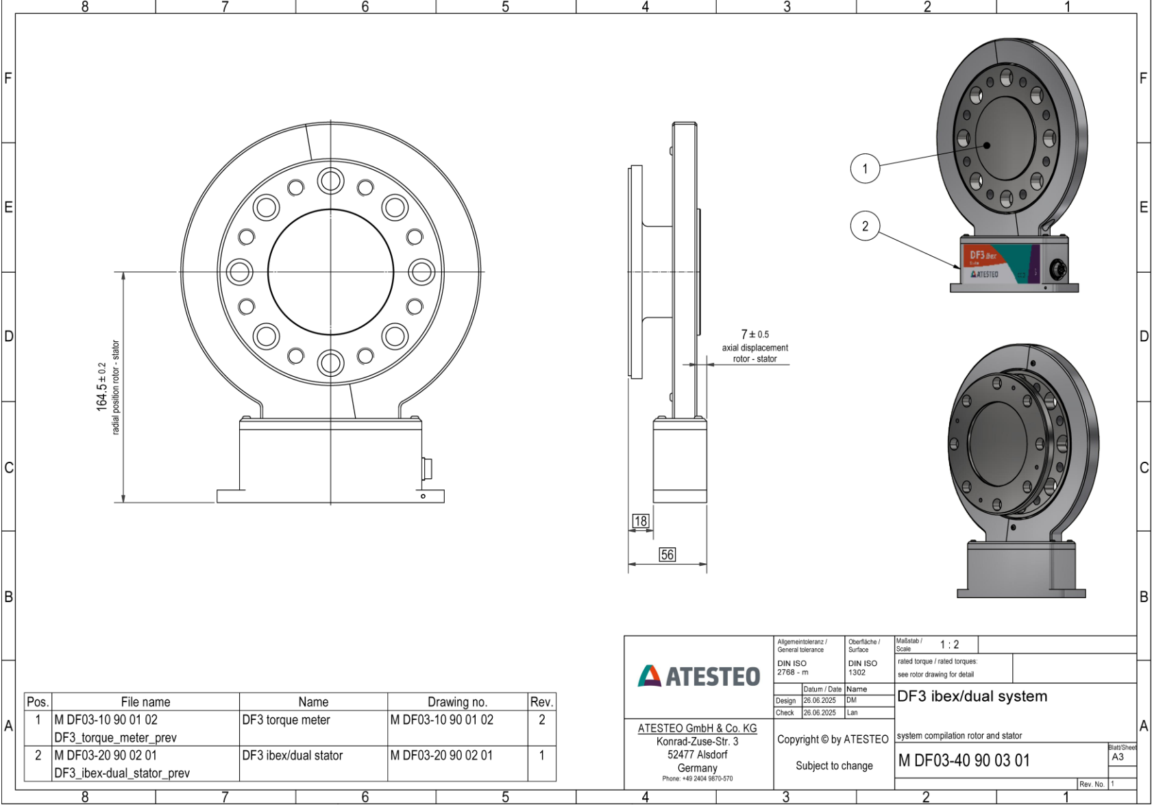
DF3 ibex - System - no speed sensor
