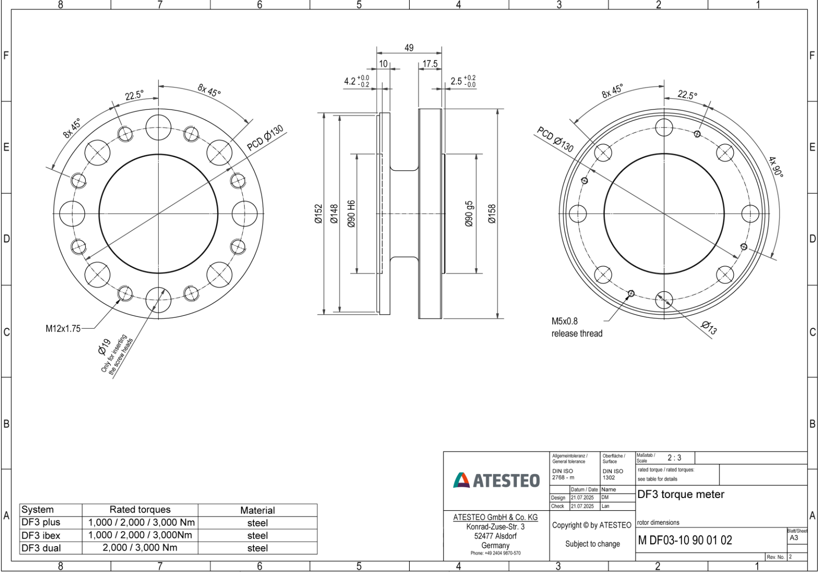
DF3 ibex - Rotor - no speed sensor
