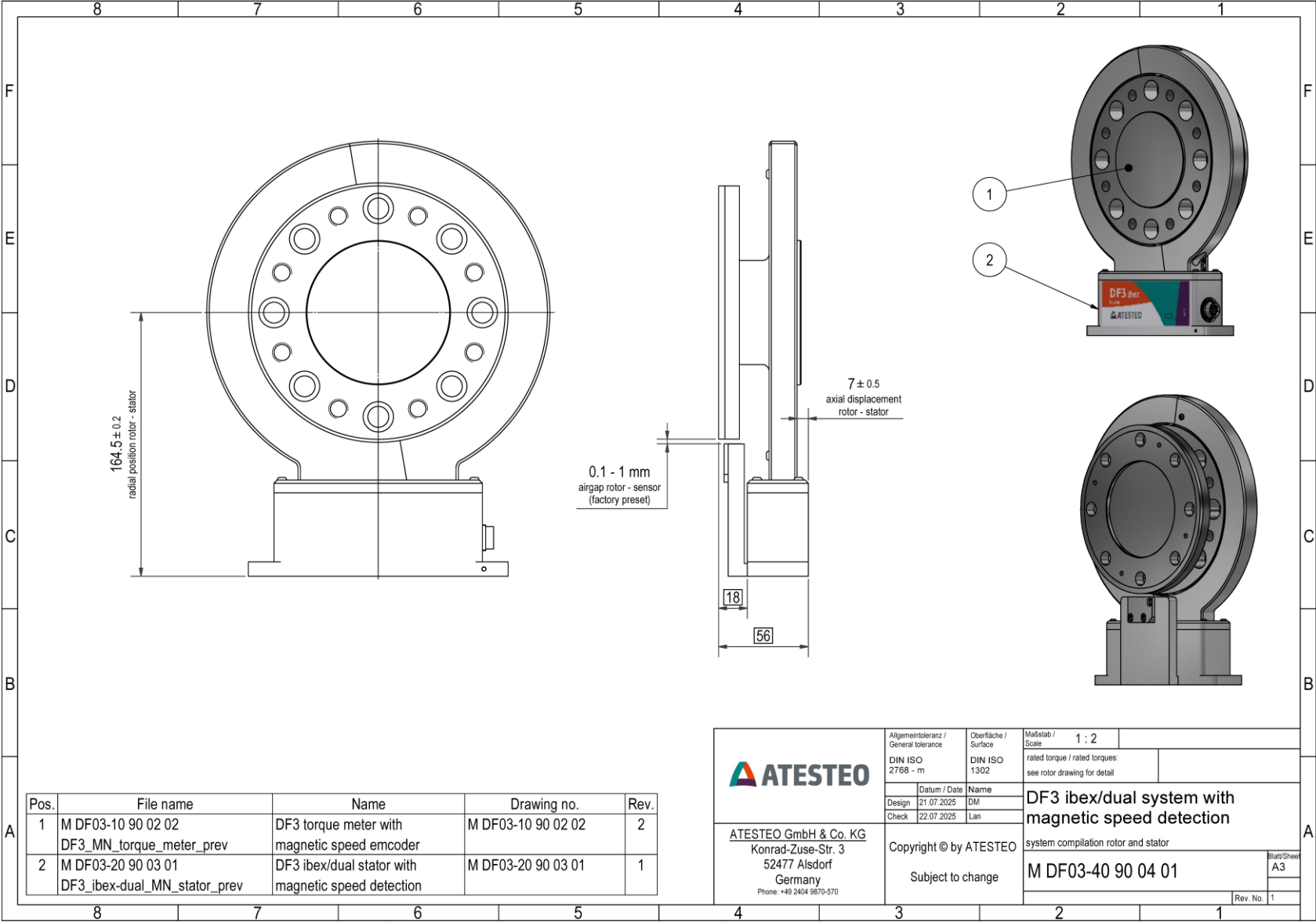
DF3 ibex - System - speed sensor
