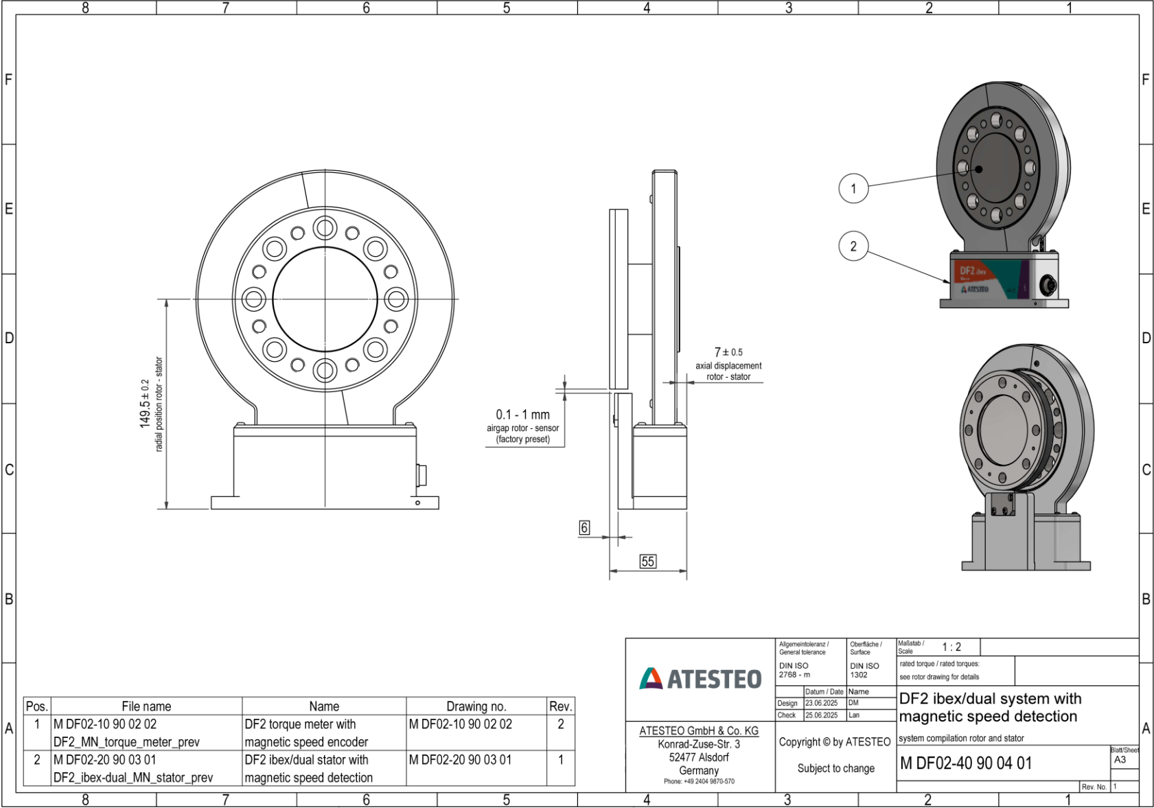
DF2 ibex - System - speed sensor
