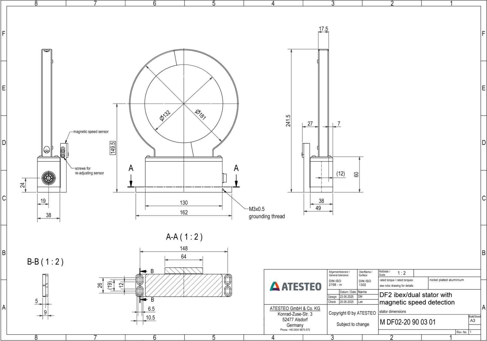
DF2 ibex - Stator - speed sensor
