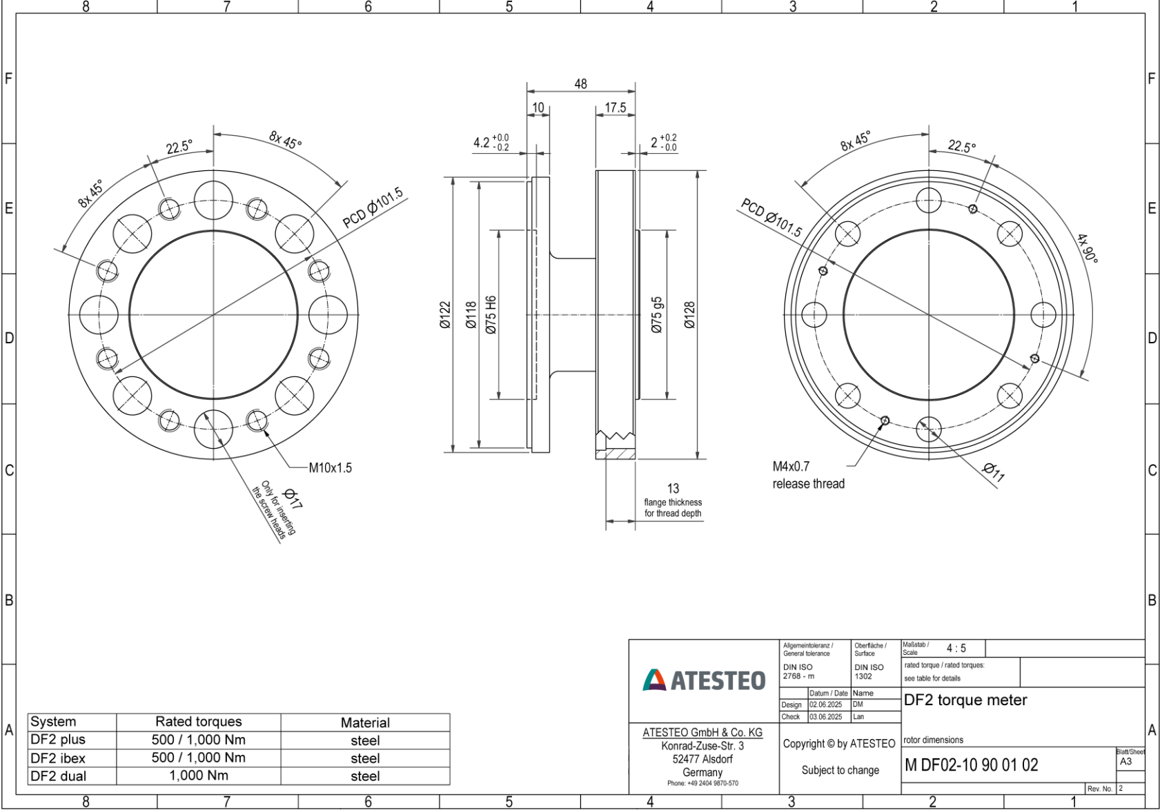
DF2 ibex - Rotor - no speed sensor
