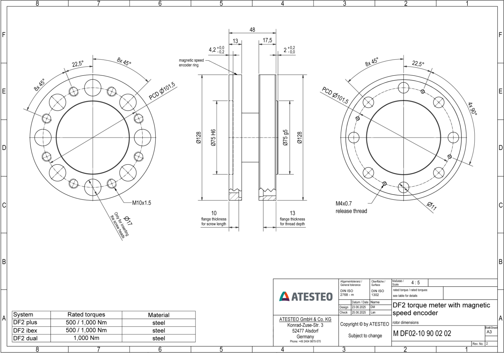
DF2 ibex - Rotor - speed sensor
