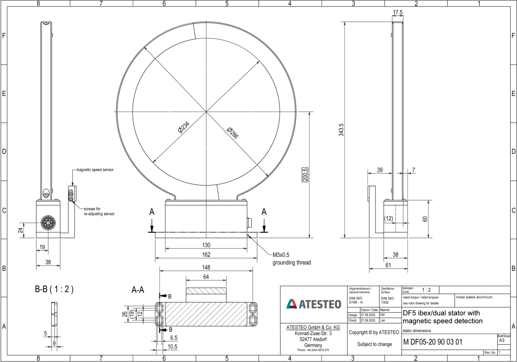
DF5 dual - Stator - speed sensor
