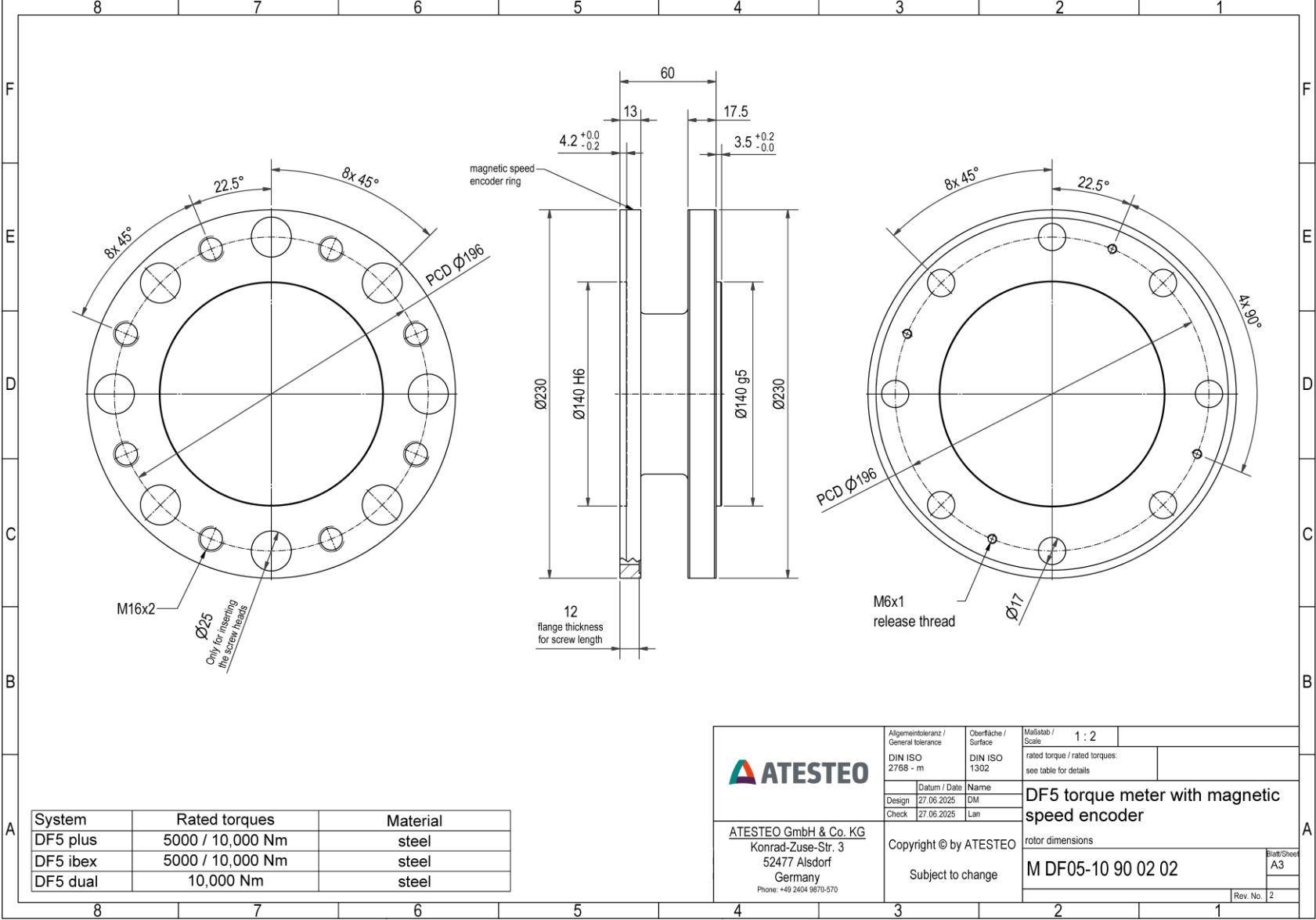
DF5 dual - Rotor - speed sensor
