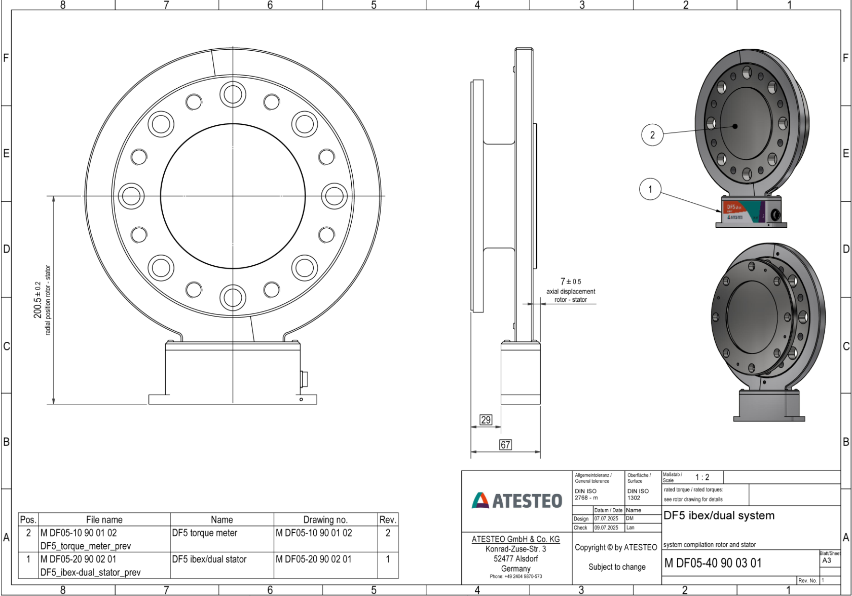
DF5 dual - System - no speed sensor
