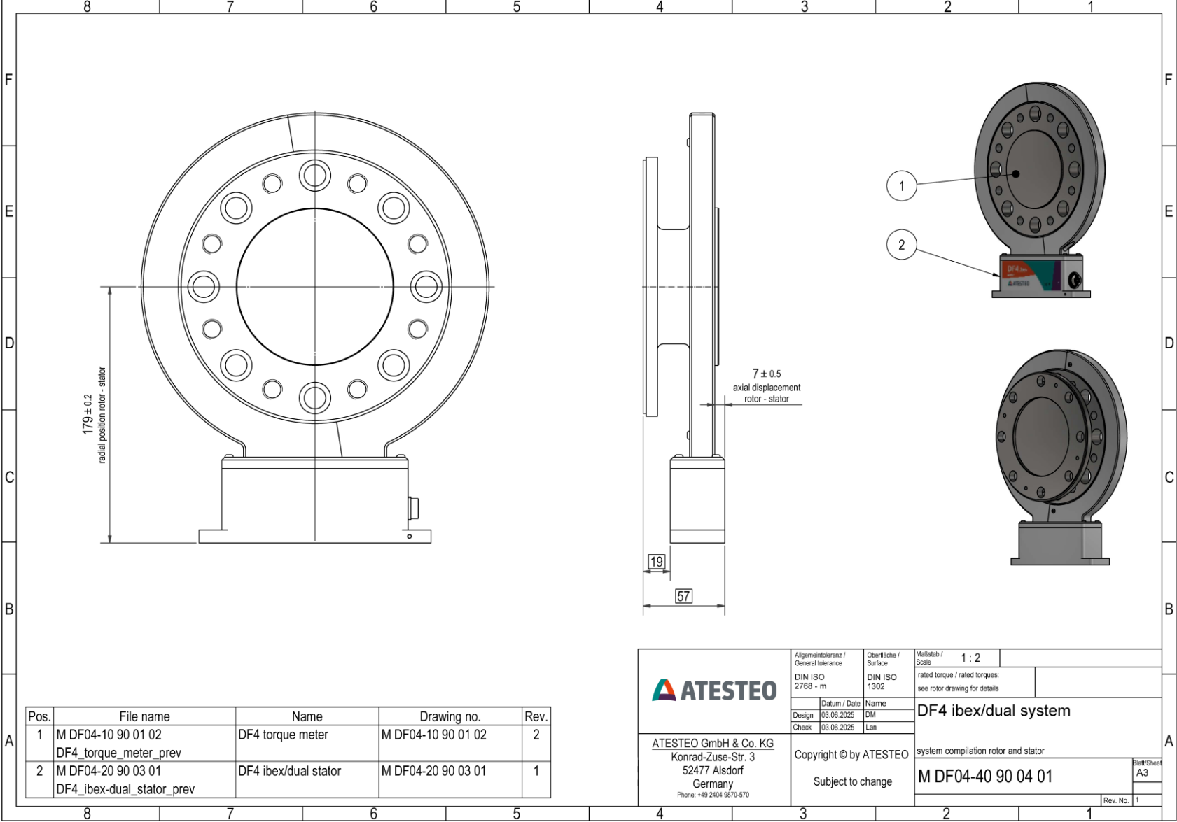
DF4 dual - System - no speed sensor
