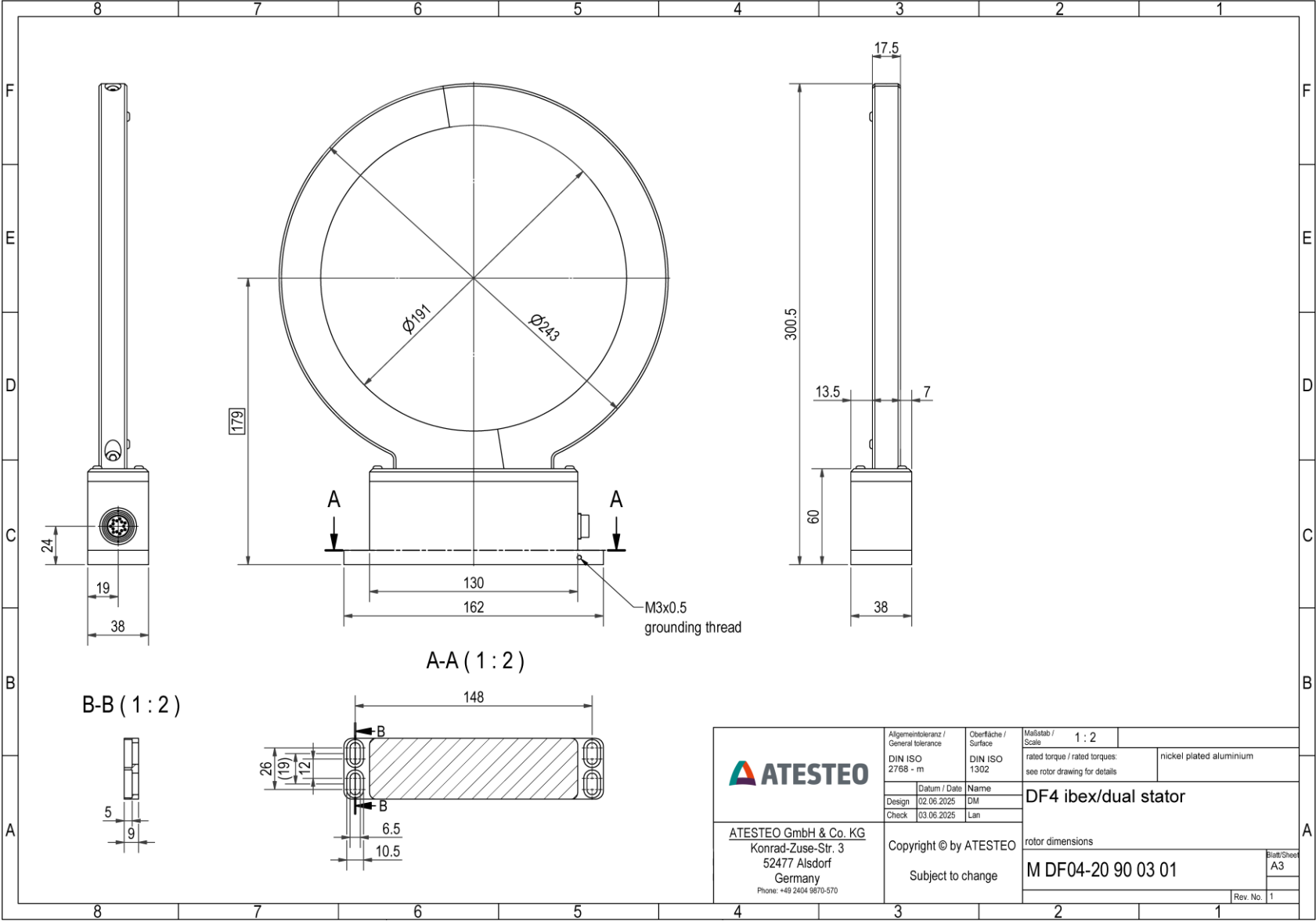
DF4 dual - Stator - no speed sensor
