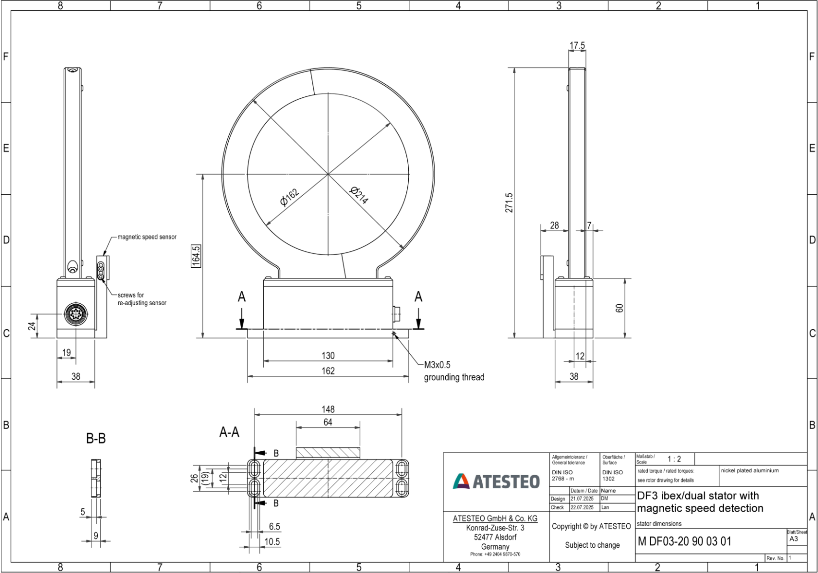
DF3 dual - Stator - speed sensor
