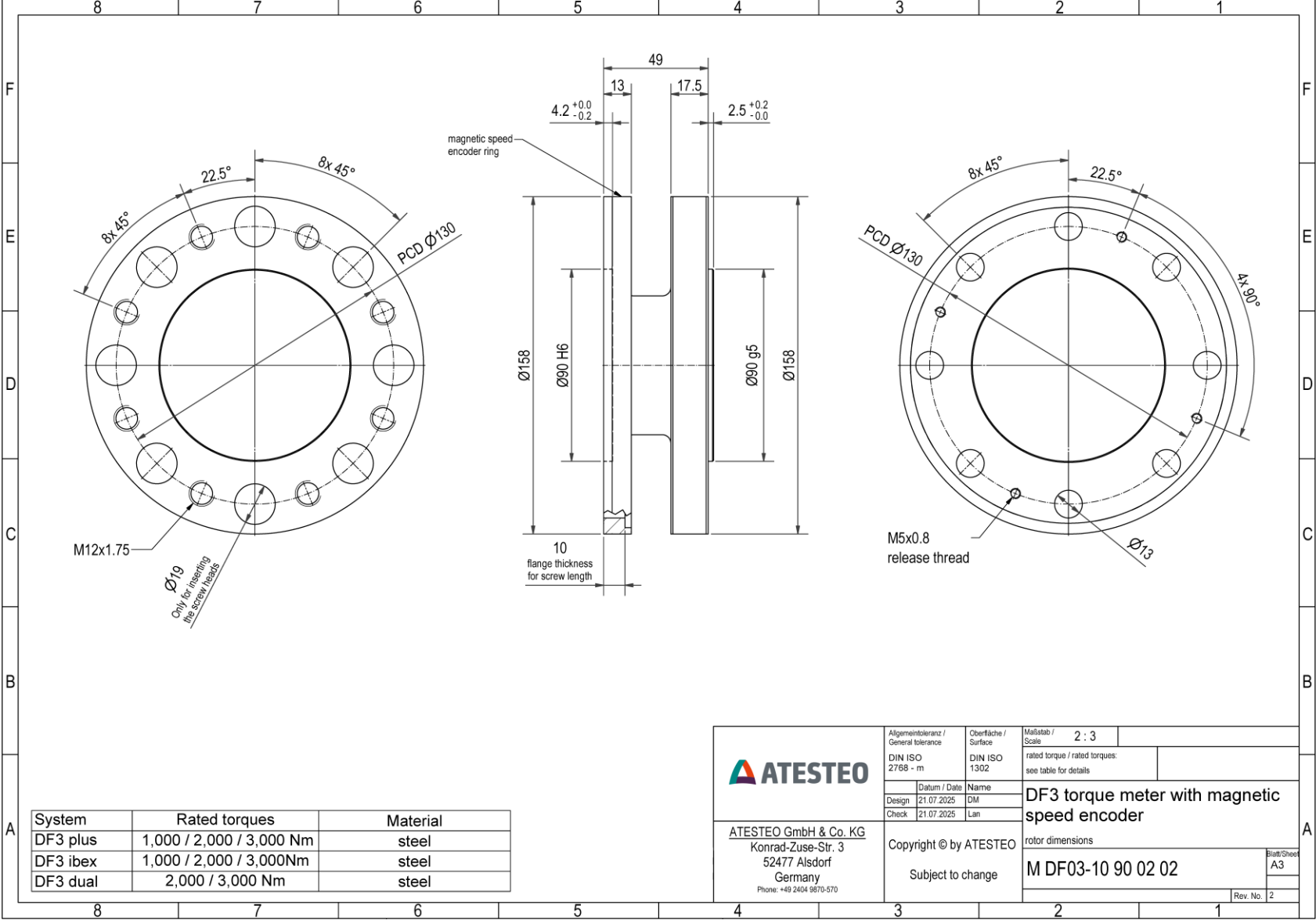
DF3 dual - Rotor - speed sensor
