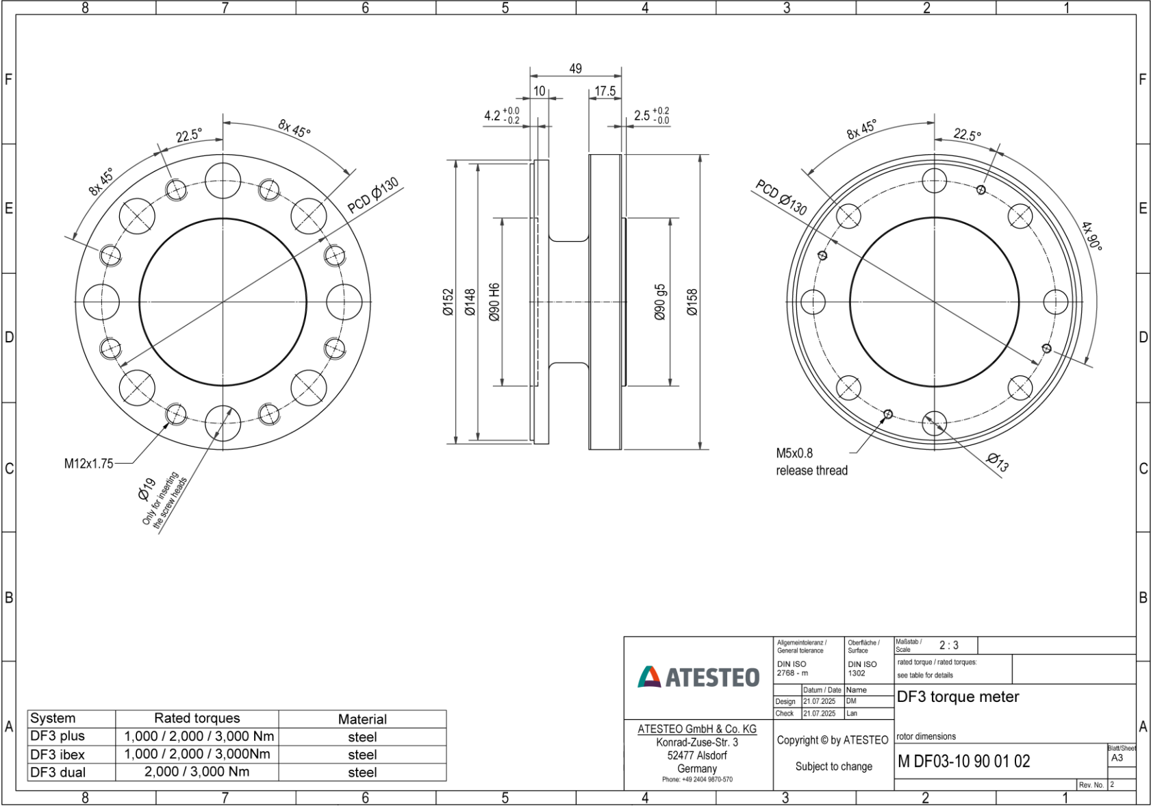
DF3 dual - Rotor - no speed sensor
