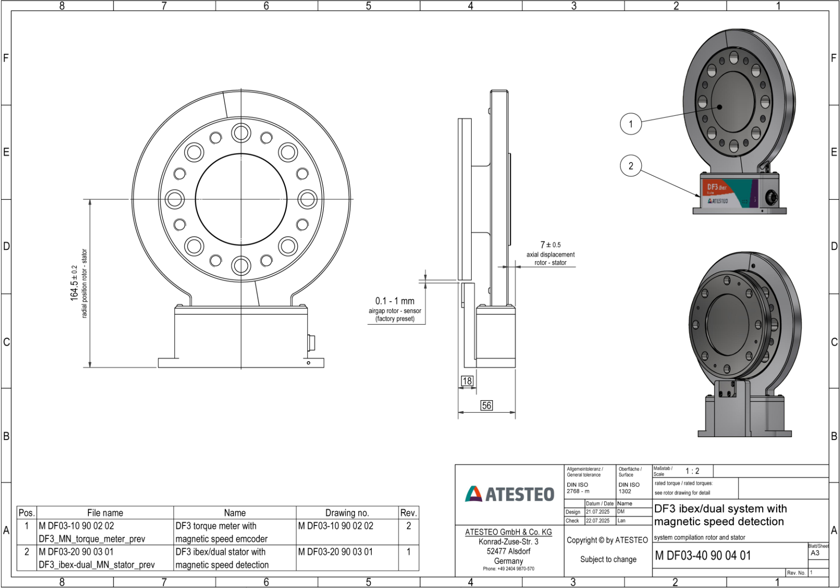
DF3 dual - System - speed sensor
