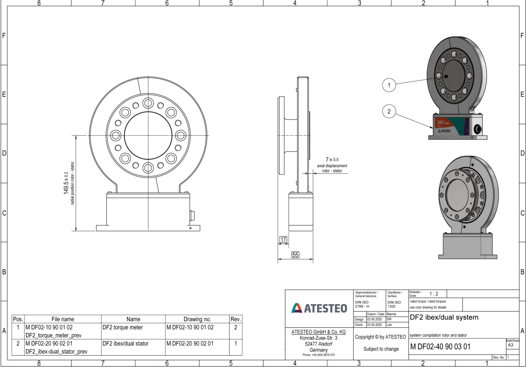
DF2 dual - System - no speed sensor
