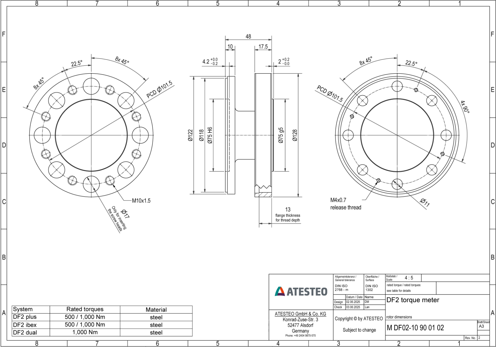
DF2 dual - Rotor - no speed sensor
