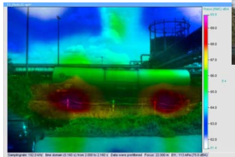
Fig. 3 Wheel emission at rolling tank wagon
