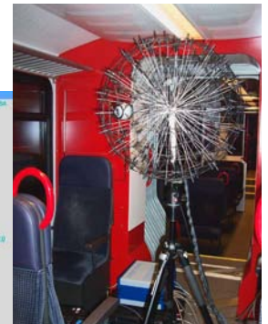
Fig. 6 Set up inside train
