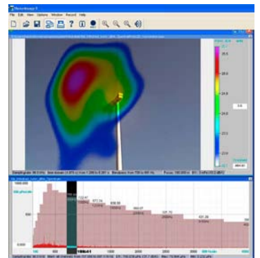
Fig. 3 Spectral Photo 2D with marked third octave band of 800 Hz and associated source locations at tip and at gear box
