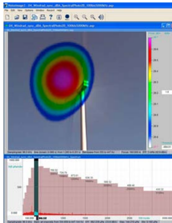
Fig. 2 Spectral Photo 2D with marked third octave band of 400 Hz and associated point of emission
