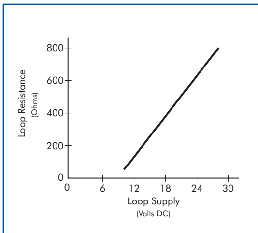
Loop Resistance vs. Minimum Loop Supply Voltage
