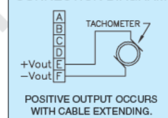
CONNECTION DIAGRAM
